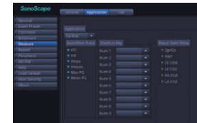
User-defined Operation
