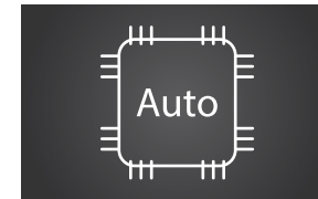
One-key Optimization
