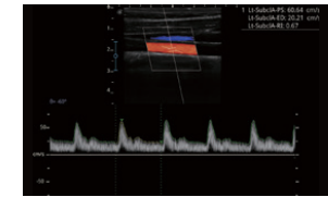
Auto Trace
