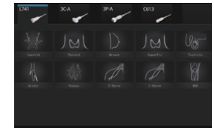
Quick Preset
